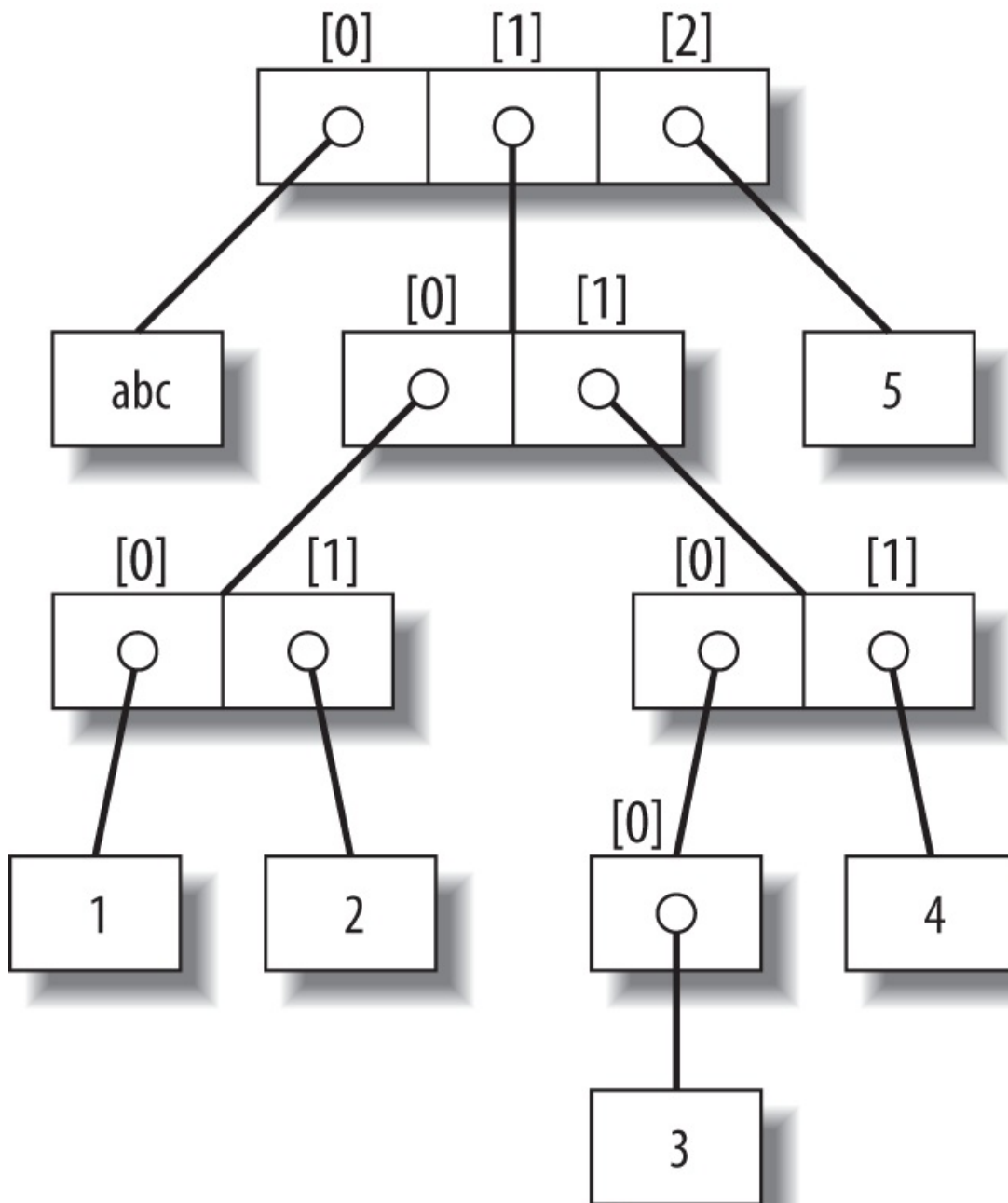
Figure 9-1. A nested object tree with the offsets of its components, created by running the literal expression ['abc', [(1, 2), ([3], 4)], 5] . Syntactically nested objects are internally represented as references (i.e., pointers) to separate pieces of memory.
