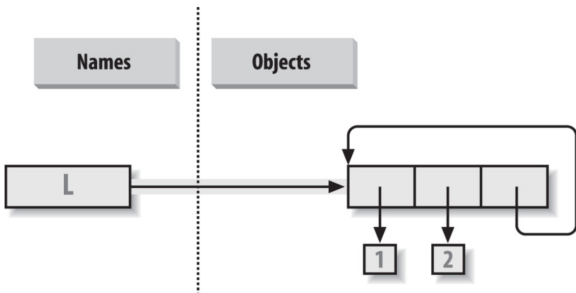
Figure D-1. A cyclic object, created by appending a list to itself. By default, Python appends a reference to the original list, not a copy of the list.
