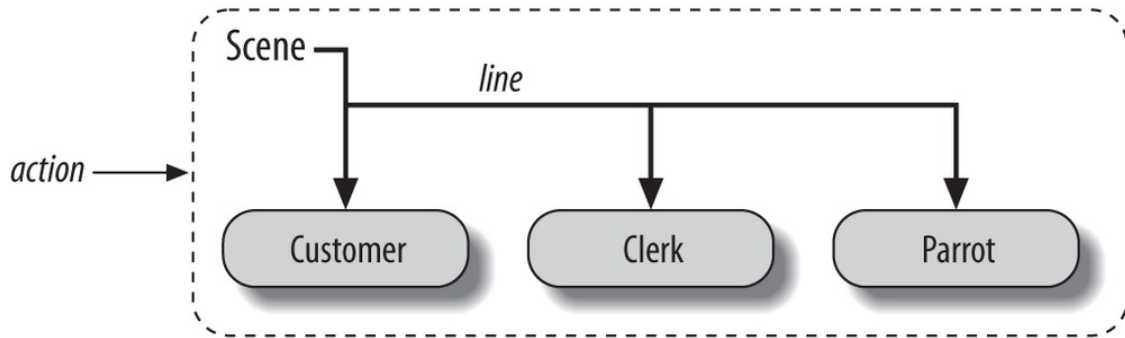
Figure 32-2. A scene composite with a controller class ( Scene ) that embeds and directs instances of three other classes ( Customer , Clerk , Parrot ). The embedded instance's classes may also participate in an inheritance hierarchy; composition and inheritance are often equally useful ways to structure classes for code reuse.
