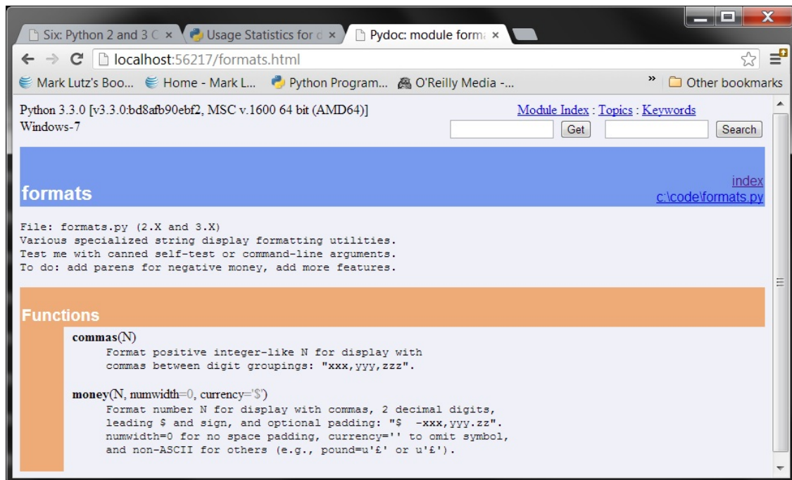
Figure 25-2. PyDoc's view of formats.py , obtained by running a "py -3 -m pydoc -b" command line in 3.2 and later and clicking on the file's index entry (see Chapter 15 )
